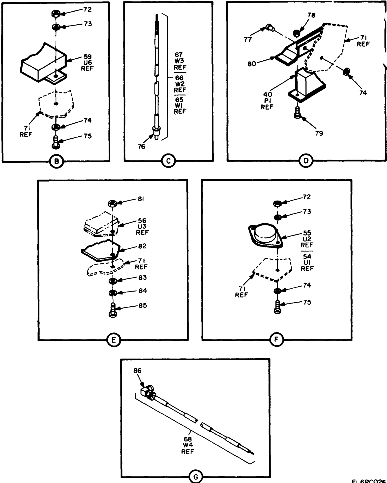
Figure 8. Main Loop Module (Sheet 3 of 3).
