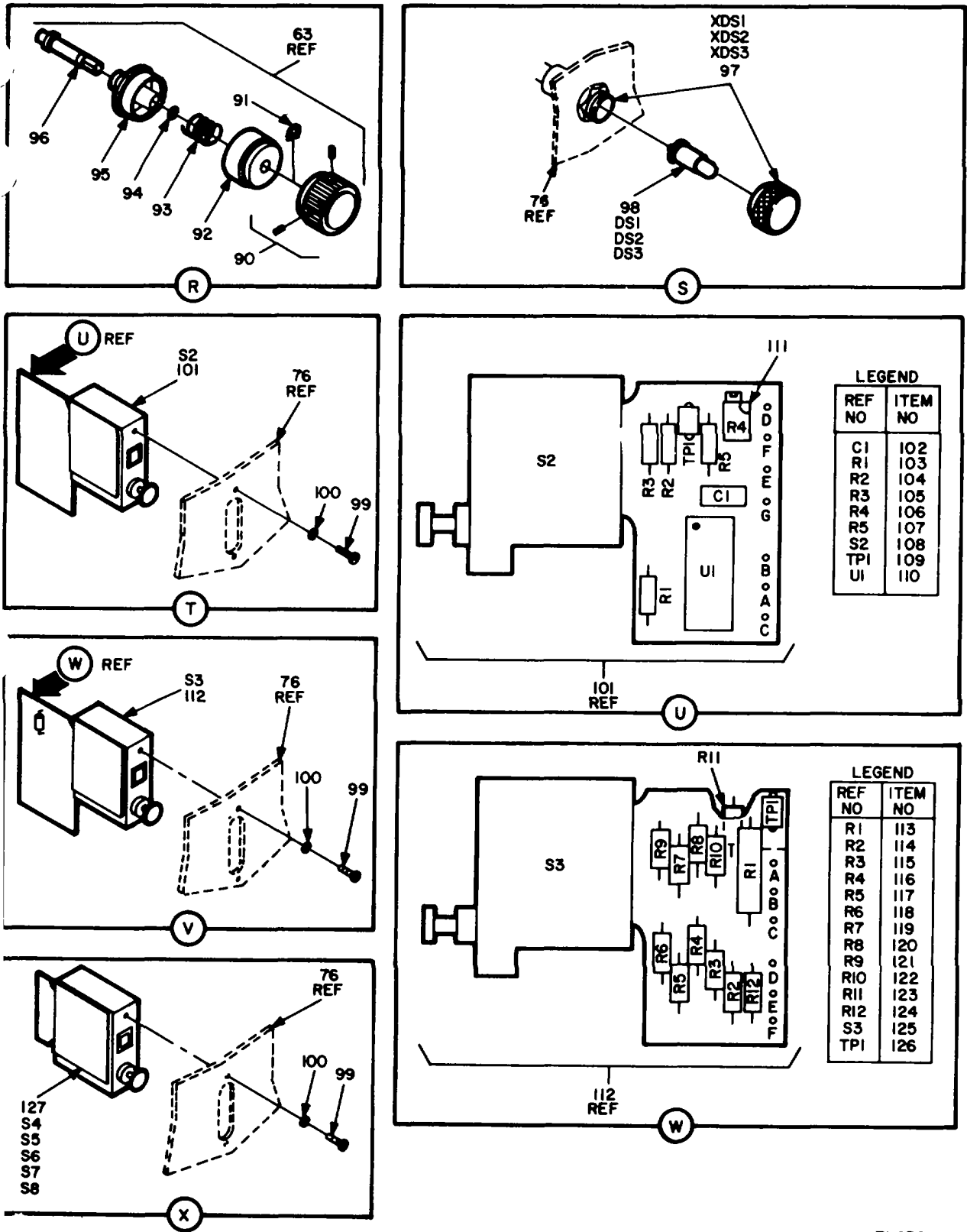
Figure 2. Electronic Frequency Synthesizer 0-1678/TSC (Sheet 5 of 6).
