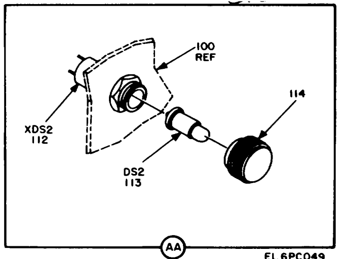
Figure 18. Electronic Frequency Converter CV-3199/TSC (Sheet 7 of 8).
