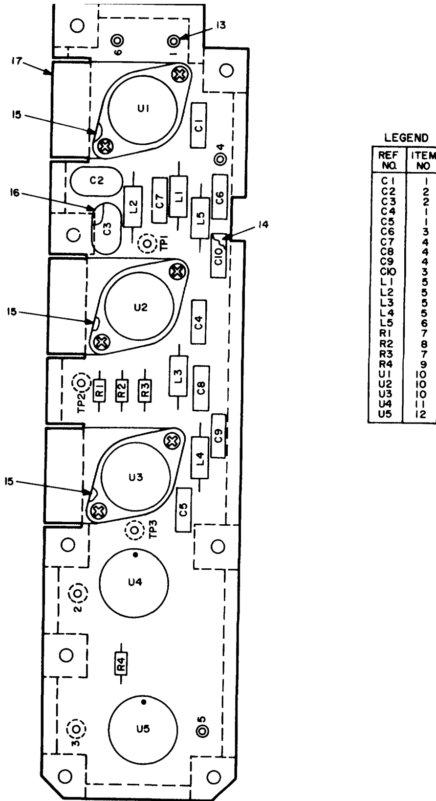
Figure 11. 70 MHz Amplifier.
