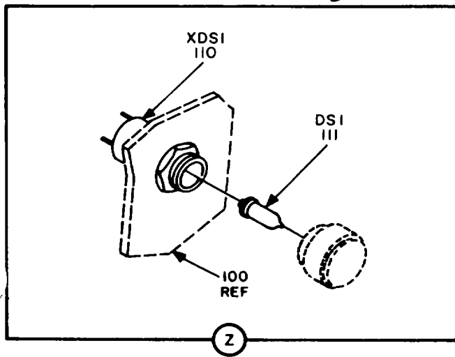
Figure 18. Electronic Frequency Converter CV-3199/TSC (Sheet 7 of 8).
