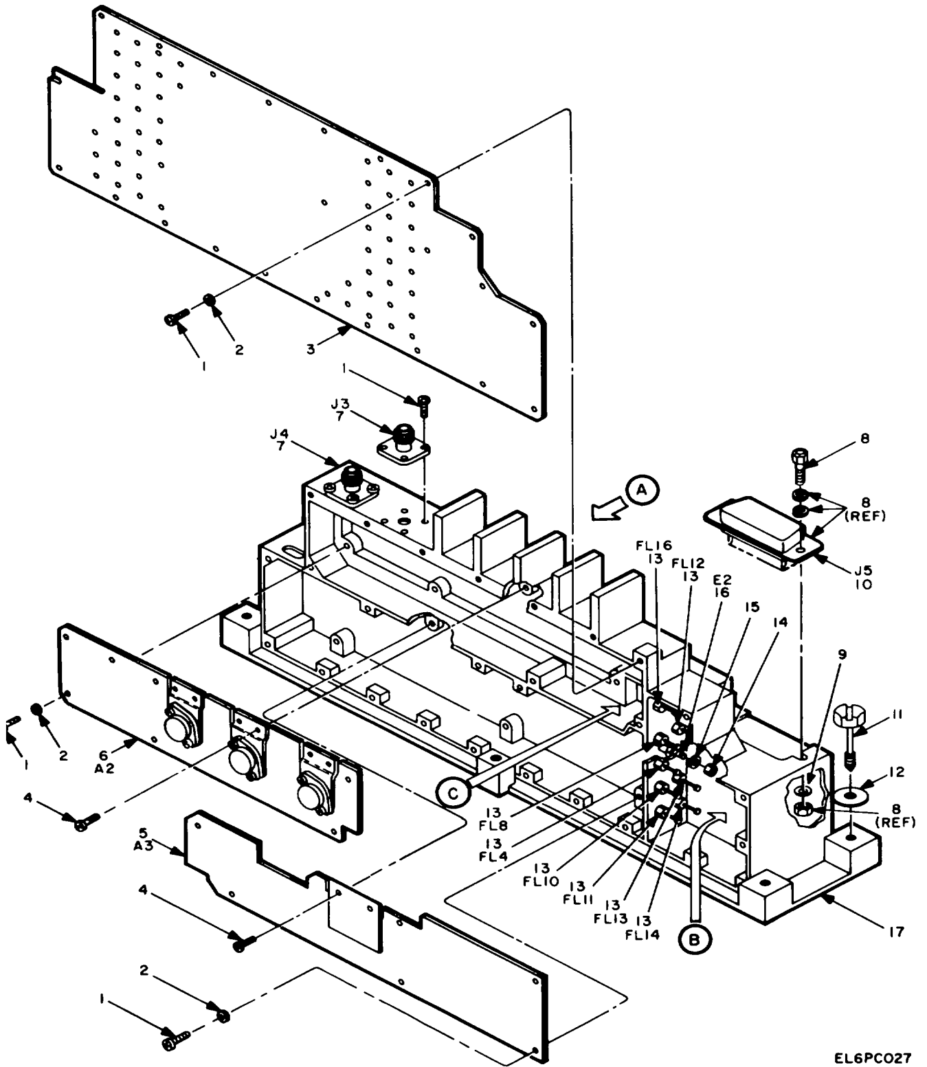
Figure 9. 70 MHz Channel (Sheet 1 of 2).
