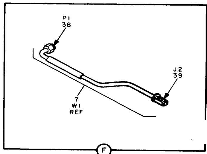
Figure 1. Electronic Frequency Converter CV-3200/TSC (Sheet 2 of 6)
