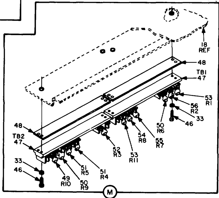
Figure 18. Electronic Frequency Converter CV-3199/TSC (Sheet 3 of 8).
