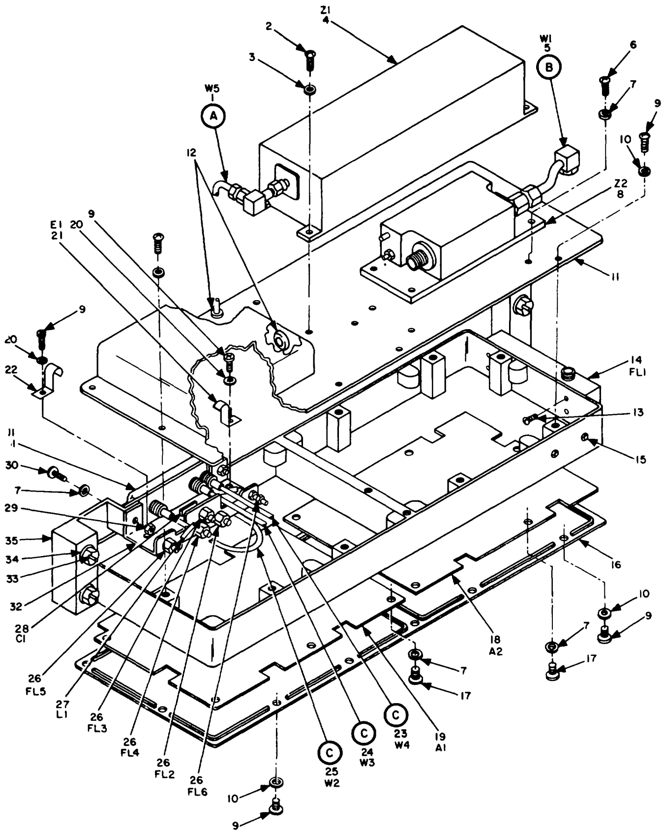
Figure 3. Fixed Frequency Generator (Sheet 1 of 2).
