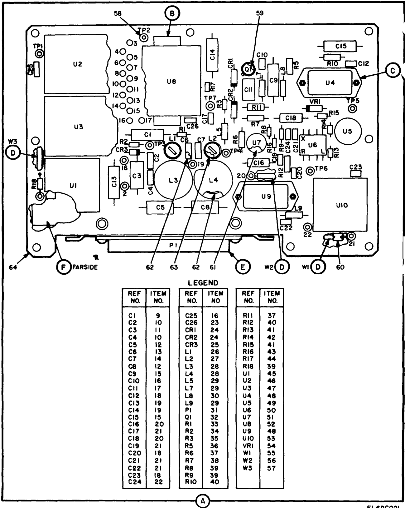
Figure 7. 1 KHz Module (Sheet 2 of 4).
