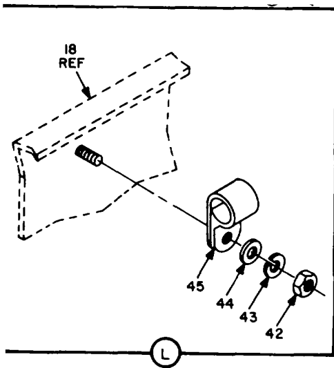
Figure 18. Electronic Frequency Converter CV-3199/TSC (Sheet 3 of 8).
