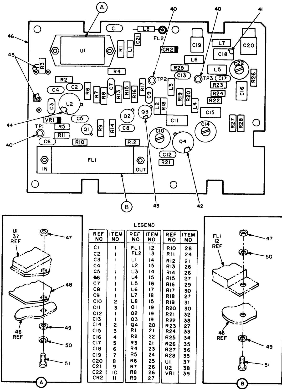
Figure 5. 630 MHz Generator.
