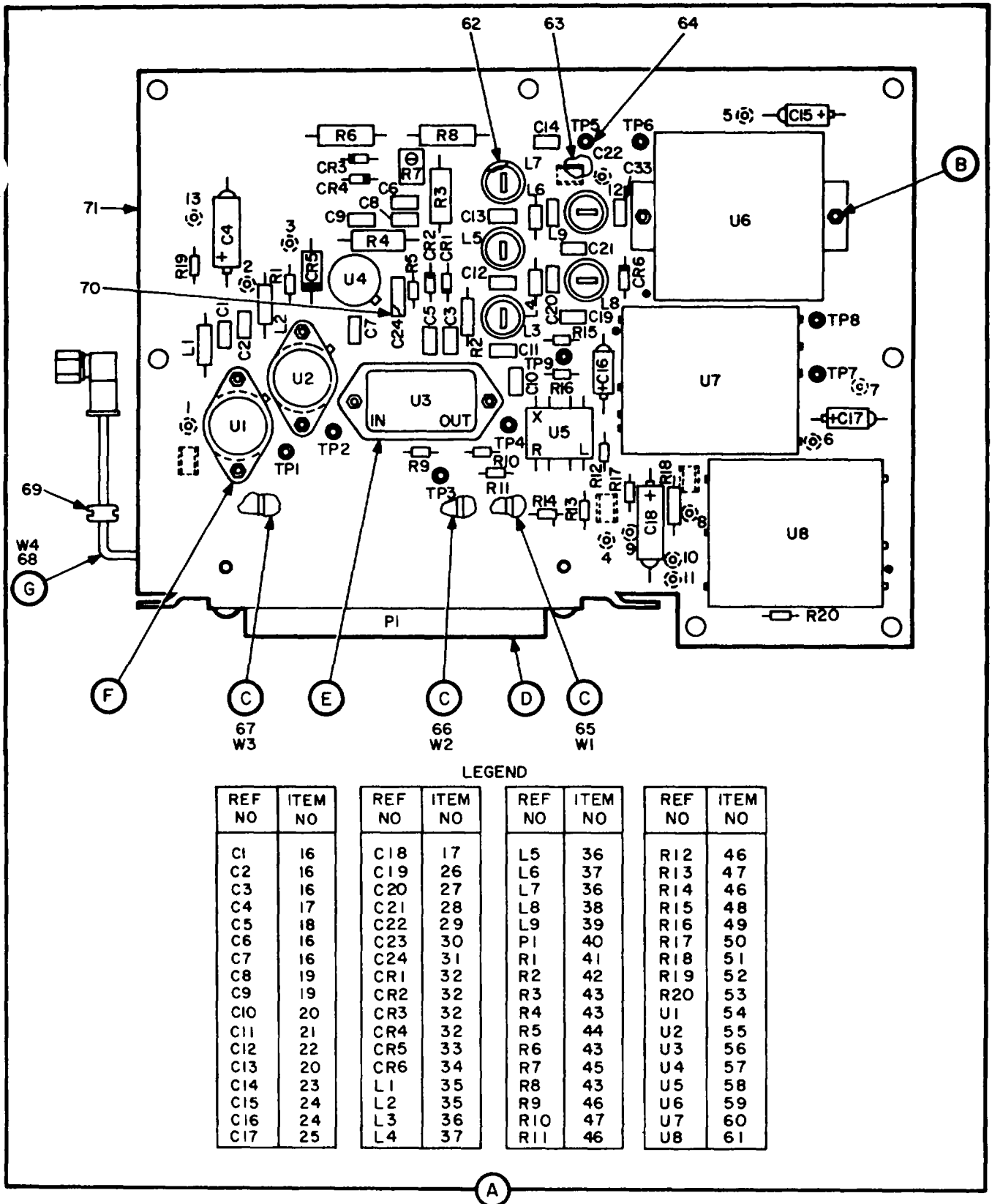
Figure 8. Main Loop Module (Sheet 2 of 3).
