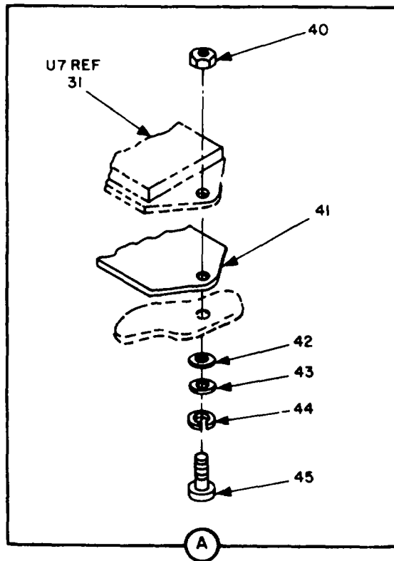
Figure 20. 70/700 MHz Mixer.
