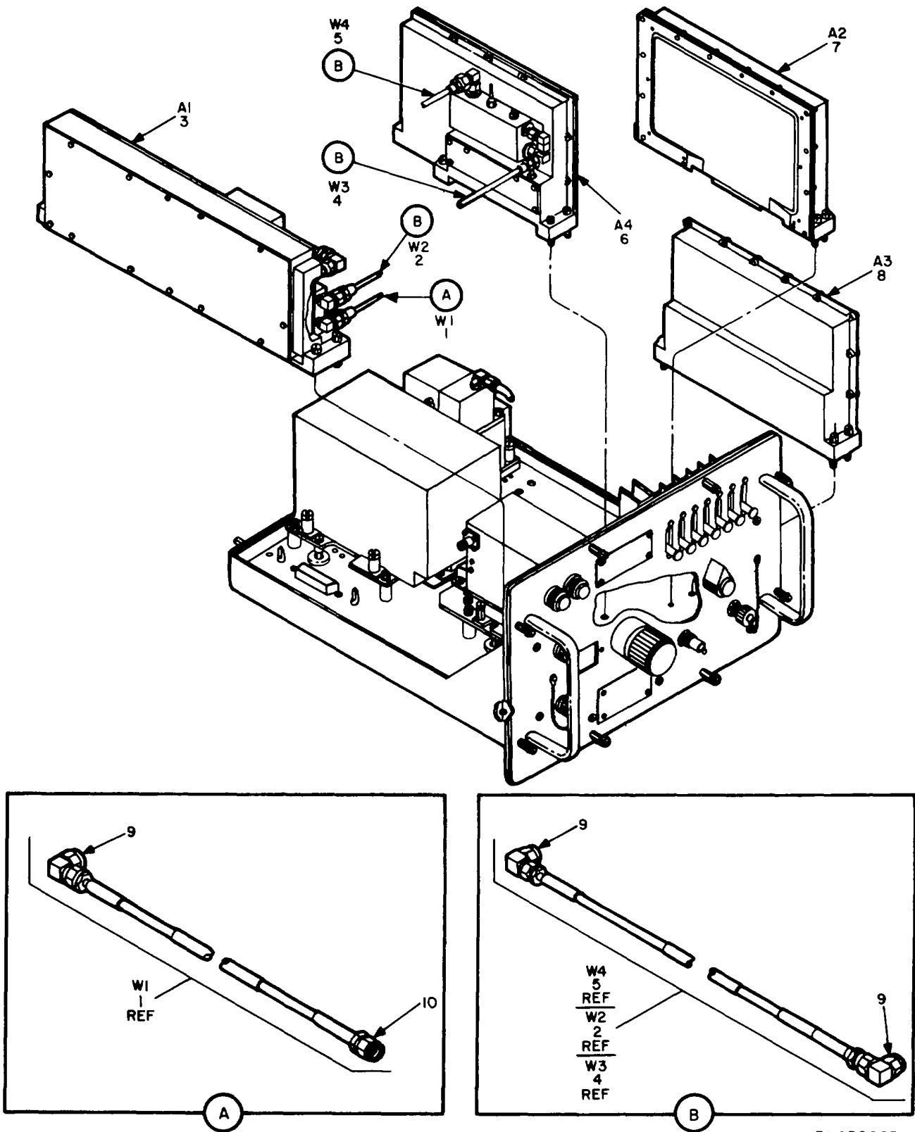
Figure 2. Electronic Frequency Synthesizer 0-1678/TSC (Sheet 1 of 6).
