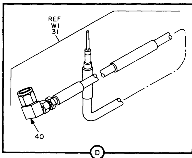
Figure 24. Filter/Monitor/IPA (Sheet 2 of 3).
