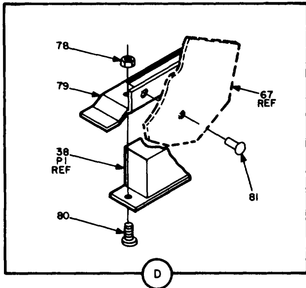
Figure 6. 1 MHz Module (Sheet 3 of 3).
