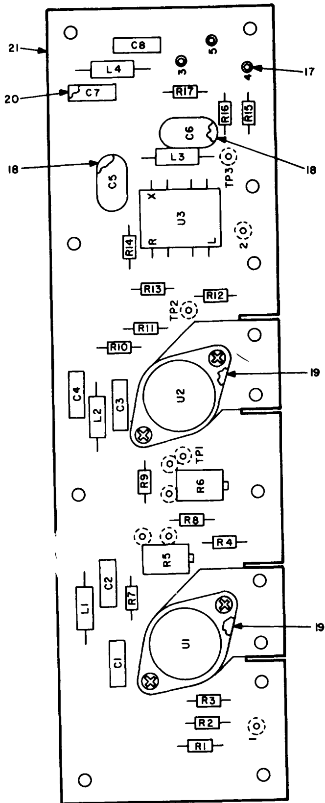
Figure 10. 700/70 MHz Mixer.
