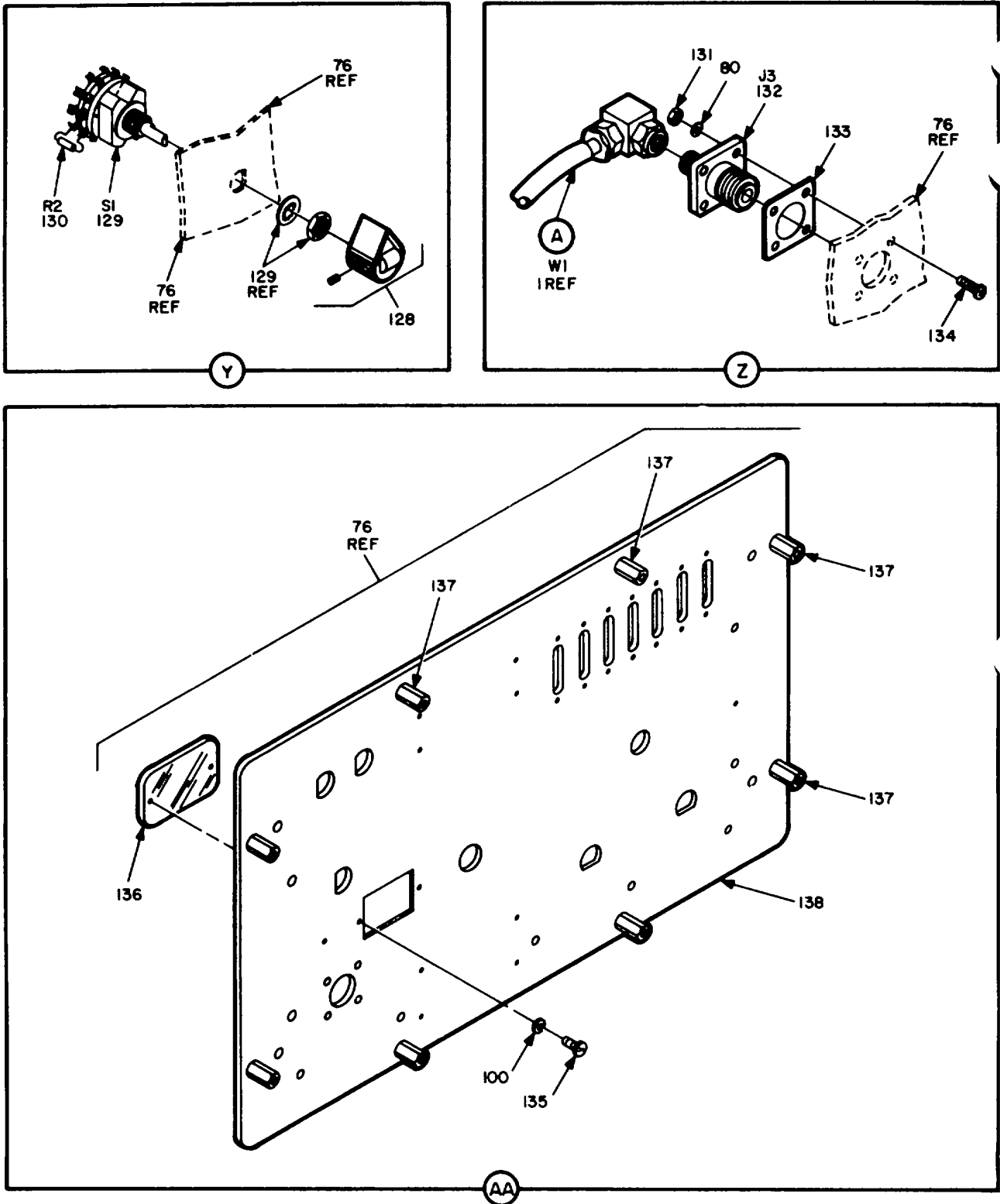
Figure 2. Electronic Frequency Synthesizer 0-1678/TSC (Sheet 6 of 6).
