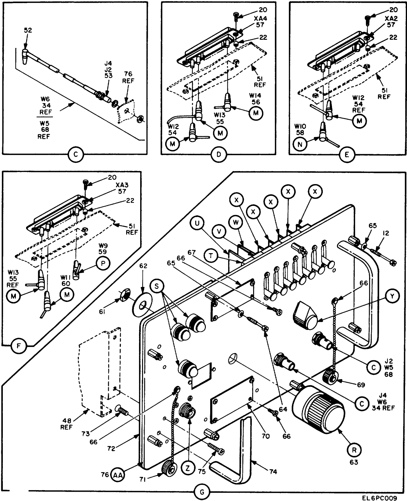
Figure 2. Electronic Frequency Synthesizer 0-1678/TSC (Sheet 3 of 6).
