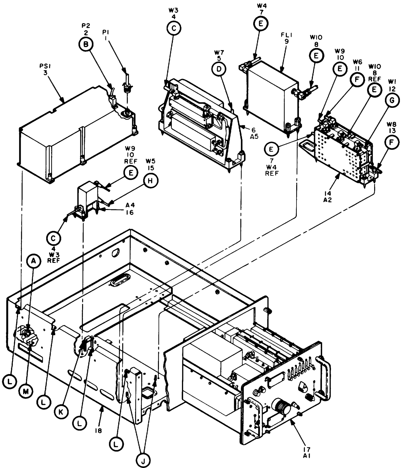
Figure 18. Electronic Frequency Converter CV-3199/TSC (Sheet 1 of 8).
