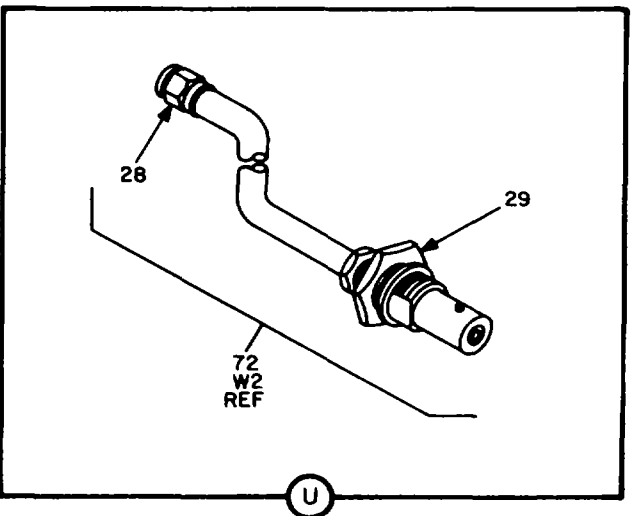
Figure 18. Electronic Frequency Converter CV-3199/TSC (Sheet 5 of 8).
